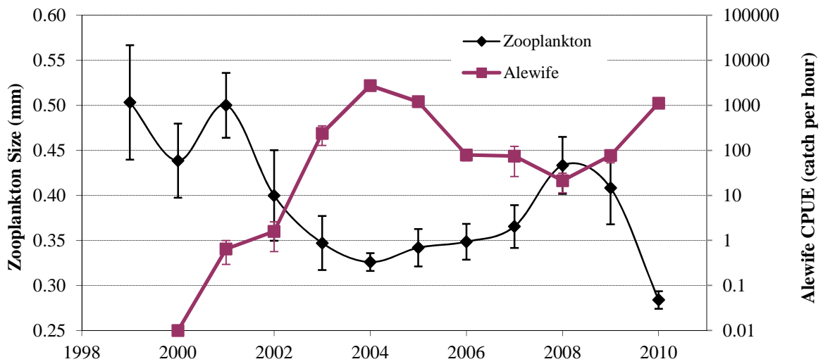
Average size of zooplankton (all taxa combined) in Onondaga Lake from April until October in 1999 to 2010 compared to annual alewife catch rates from electrofishing from 2000-2010. Note: error bars are standard error.
