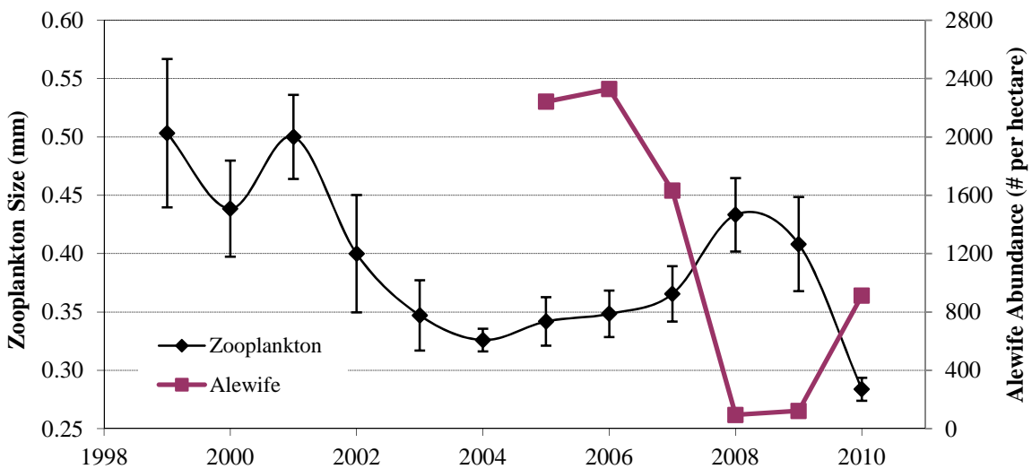
Average size of zooplankton (all taxa combined) in Onondaga Lake from April until October in 1999 to 2010 compared to annual alewife abundance estimates from hydroacoustic surveys conducted in June from 2005-2010. Note: error bars are standard error. Hydroacoustics report indicates that 2008 and 2009 alewife abundance is likely overestimated due to interference from bubbles.
