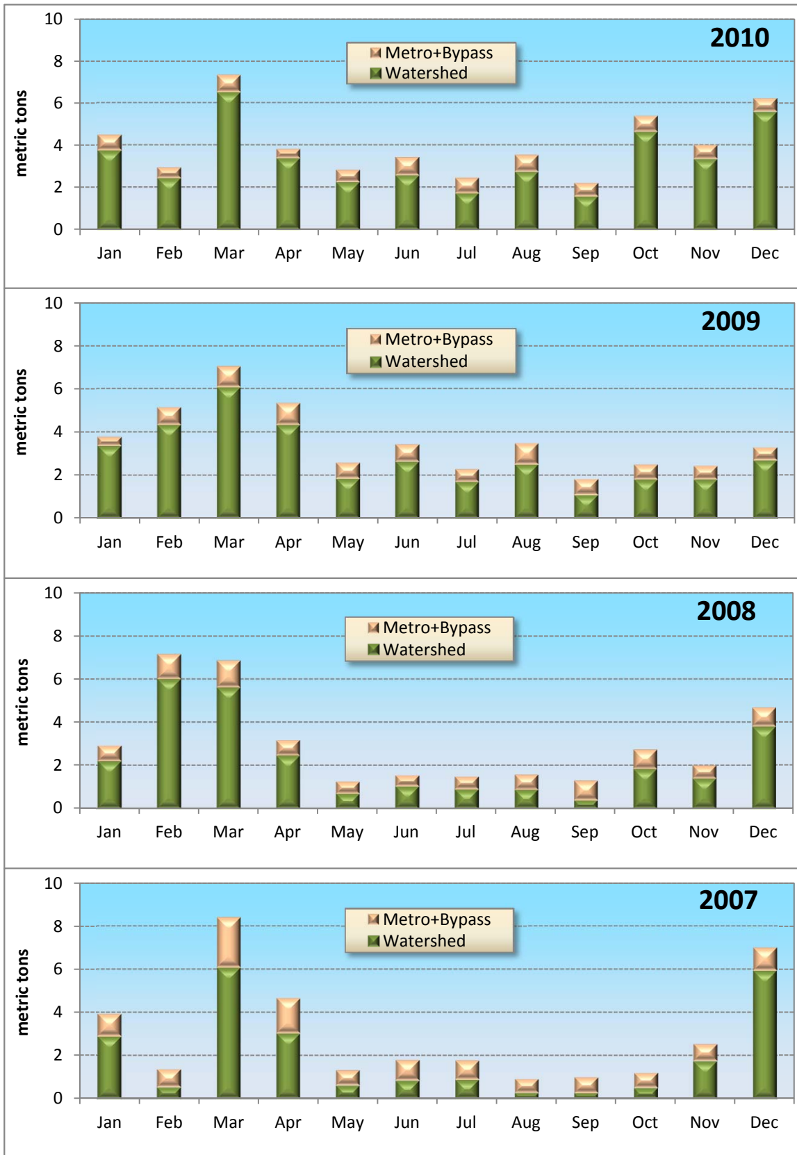
Sum of the monthly loading for total phosphorus to Onondaga Lake, 2007 to 2010. Summer loadings are lower during dry years than during wet years. Metro's ActiFlo phosphorus treatment came on-line in 2005.
