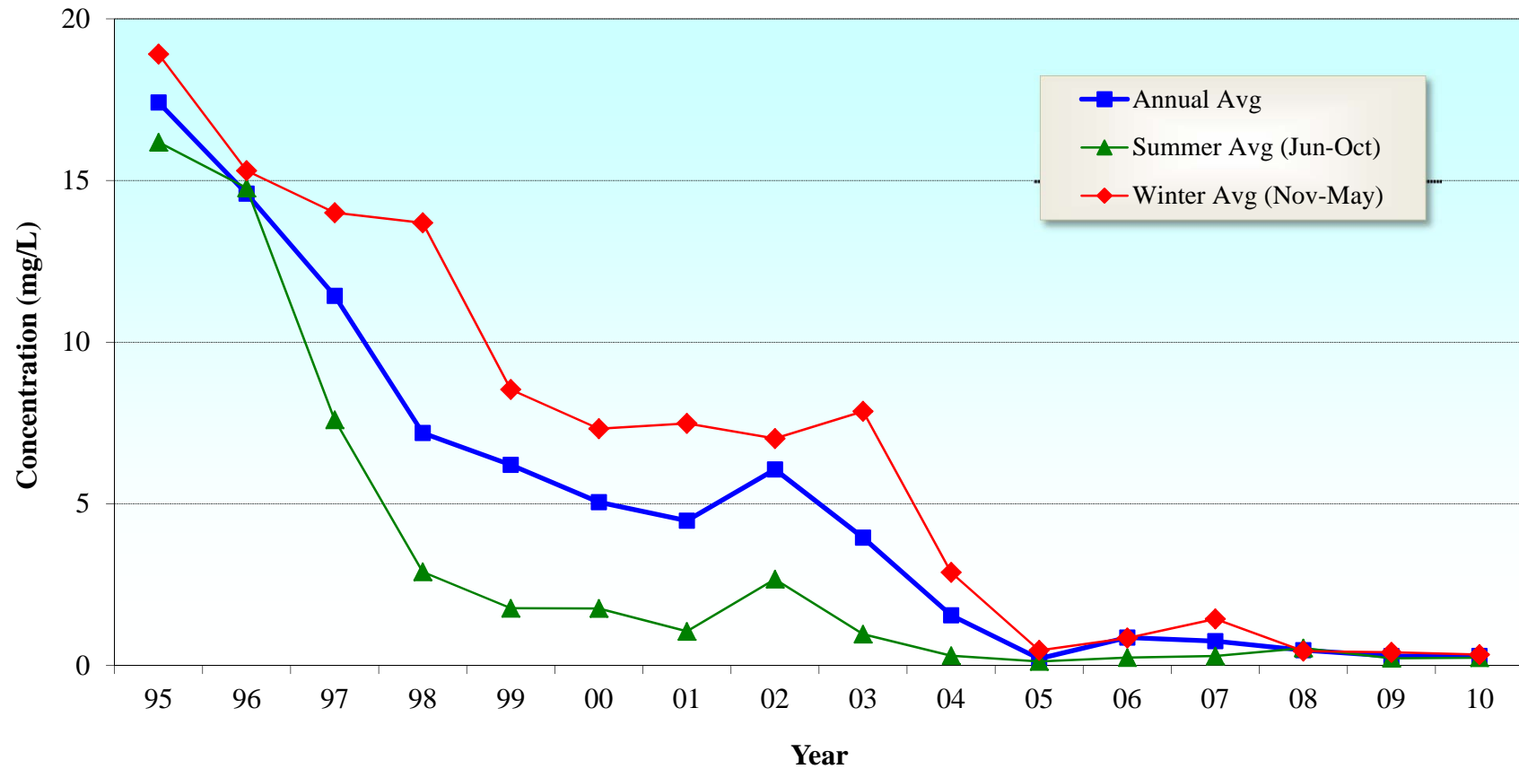
Seasonal average ammonia-N concentration in Metro Outfall 001 effluent over time. The BAF treatment system went on-line in January 2004.
