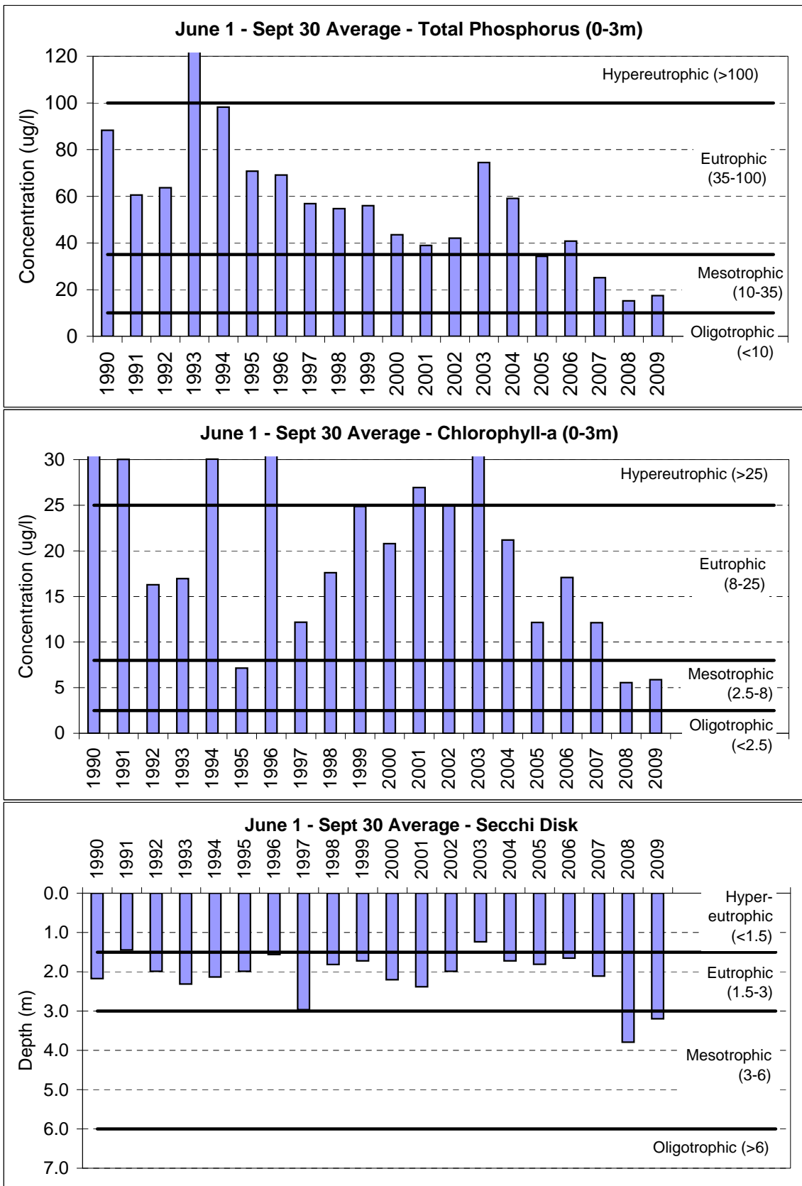
Three indicators of trophic status - phosphorus, chlorophyll-a, and transparency - shown over time (1990-2009), using data collected at South Deep Station in Onondaga Lake.
