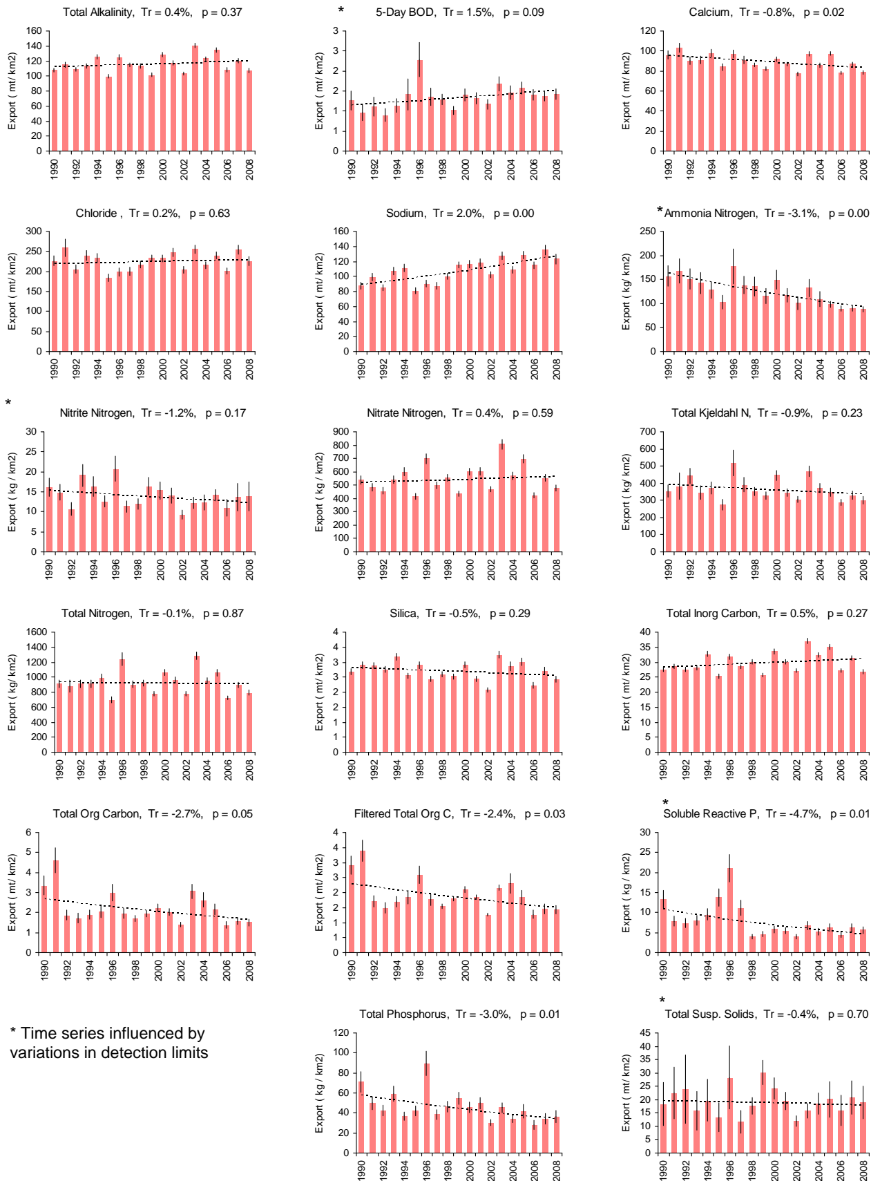
Figure 6 Trends in Rainfall-Adjusted NonPoint Loads by Variable, 1990-2008
