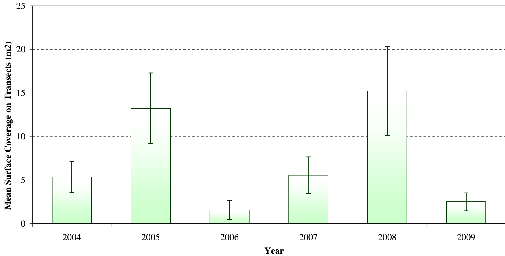
Mean macroalgae abundance, with standard error, at nine nearshore sample locations in Onondaga Lake from 2004 to 2009.
