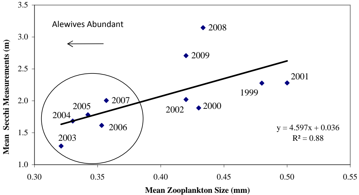
A) Mean Secchi disk measurements and mean zooplankton size from April through October in Onondaga Lake, 1999 to 2009. B) Regression of mean Secchi disk measurements and mean zooplankton size from April through October in Onondaga Lake 1999 to 2009, labels are the year.
