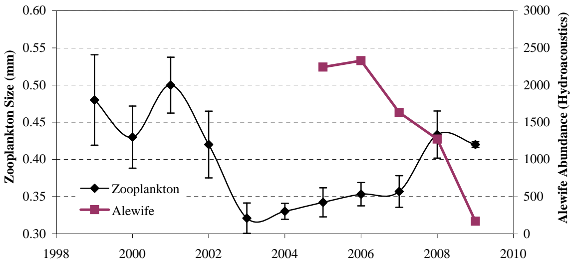
Average size of zooplankton (all taxa combined) in Onondaga Lake from April until October in 1999 to 2009 compared to annual alewife abundance estimates from hydracoustic surveys conducted in June from 2005-2009.
