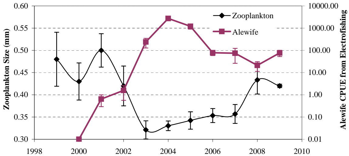
Average size of zooplankton (all taxa combined) in Onondaga Lake from April until October in 1999 to 2009 compared to annual alewife catch rates from electrofishing from 2000-2009.
