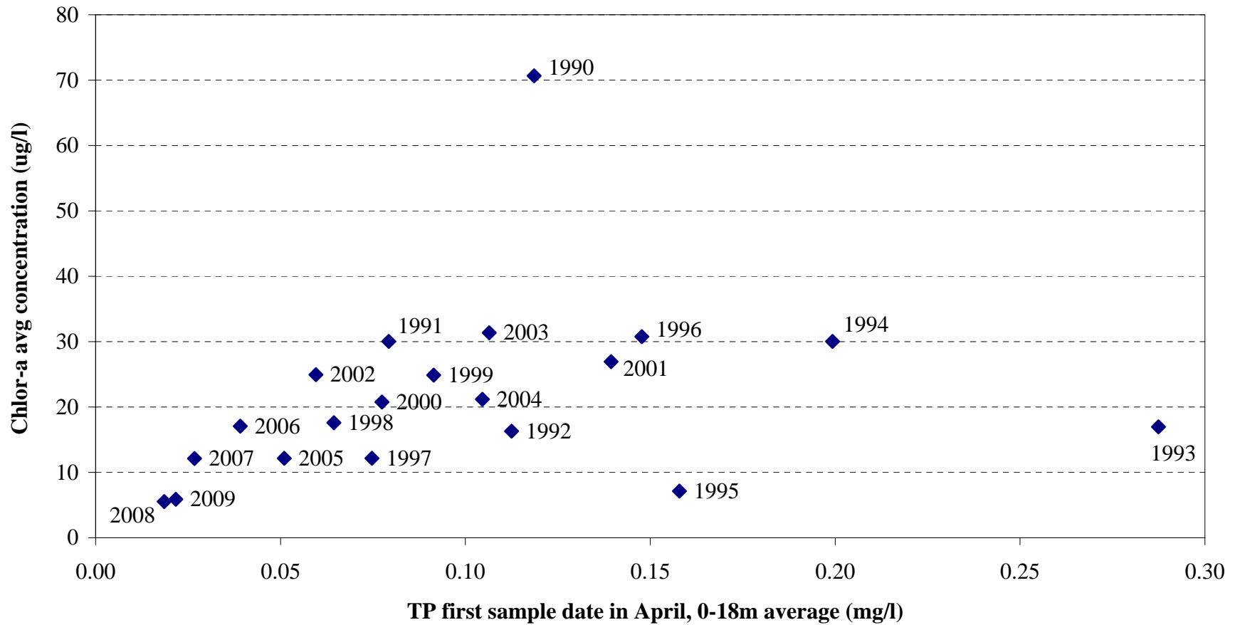
Relationship 1990 to 2009 between spring total phosphorus (TP) concentration (averaged across sample depths from 0 to 18 meters) and summertime chlorophyll-a concentrations at South Deep station in Onondaga Lake. Summertime is defined as the period from June 1 through September 30.
