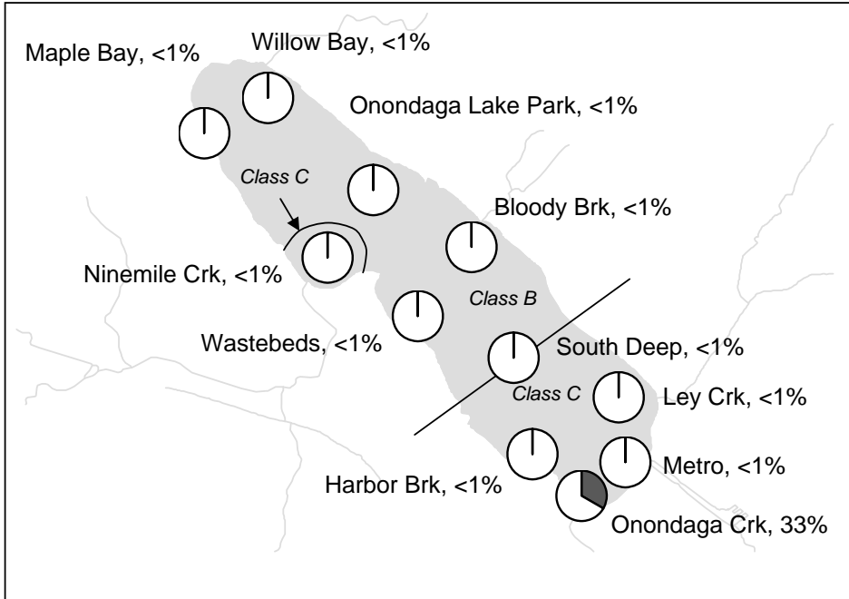
Nearshore and South Deep fecal coliform bacteria results in 2009. Shaded area of pie charts and percents indicate the percent of monthly geometric means that exceeded 200 cells per 100 ml for the disinfection period April 1 through October 15.
