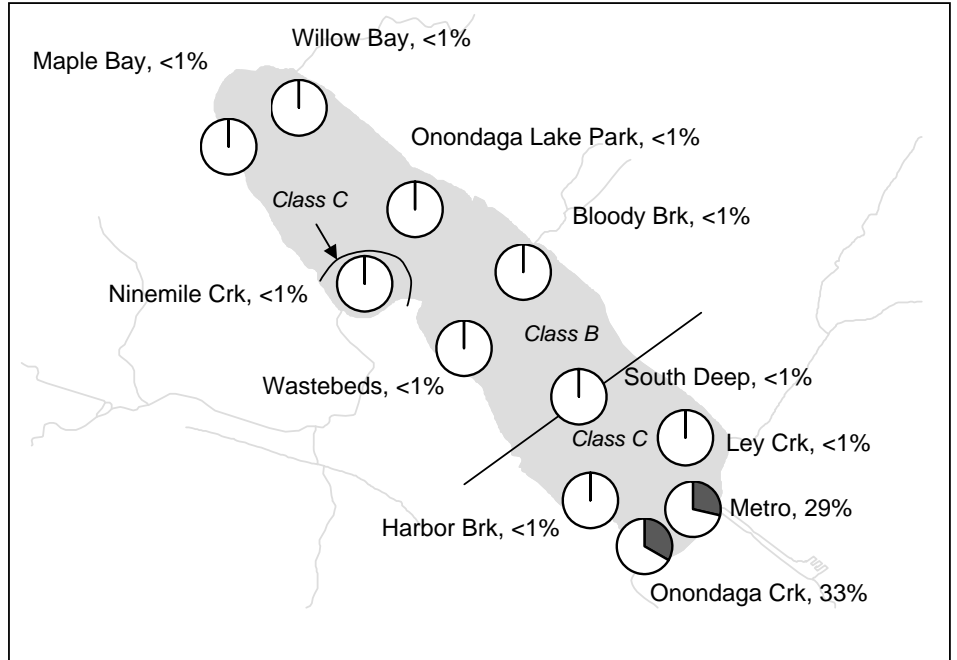
Nearshore and South Deep E. coli results in 2009. Shaded area of pie charts indicates percent of monthly geometric means that exceeded 126 cells per 100 ml for the disinfection period April 1 through October 15.
