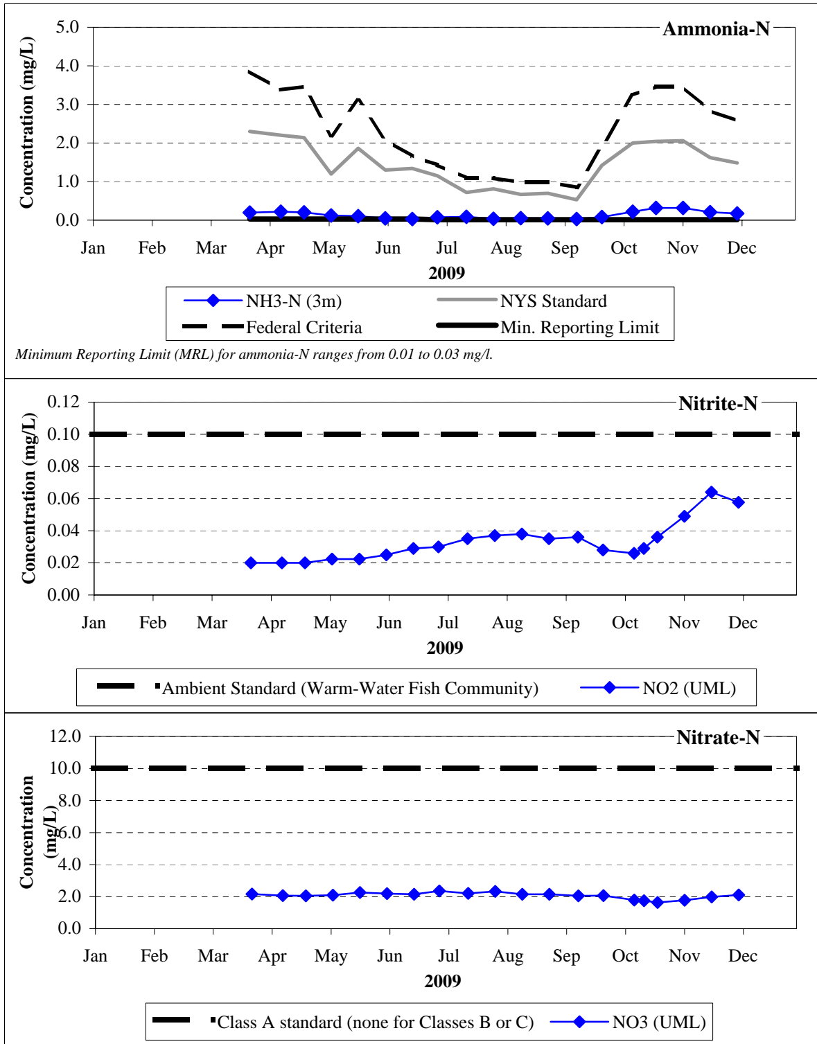
2009 concentrations of ammonia-N (3-meter depth), nitrite-N (UML) and nitrate-N (UML) at the Onondaga Lake South Deep Station, compared with applicable federal and/or state water quality standards and/or criteria. UML - Upper Mixed Layer .
