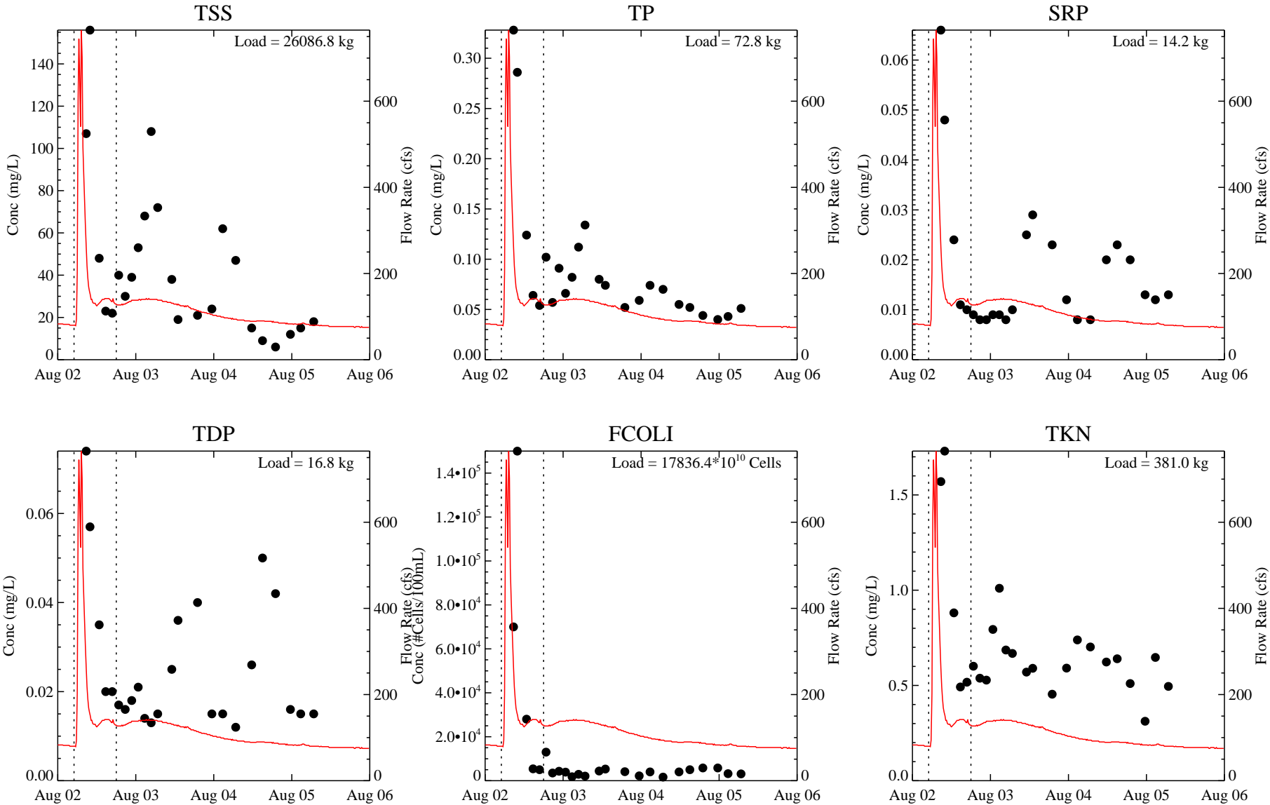
Temporal plot of storm survery data collected by OCDWEP and 15-minute flows recorded by USGS in Onondaga Creek at Spencer St in August 2009.
