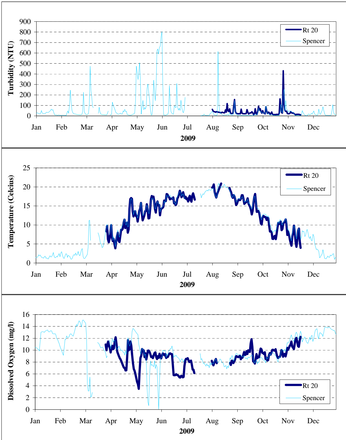
Daily average in-situ sonde results in 2009 for turbidity, temperature and dissolved oxygen at Spencer Street (downstream) and Route 20 (upstream) stations on Onondaga Creek. Daily averages calculated from 15-minute interval data.
