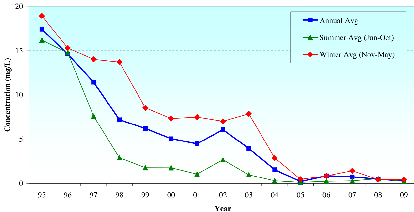
Seasonal average ammonia-N concentration in Metro Outfall 001 effluent over time. The BAF treatment system went on-line in January 2004.
