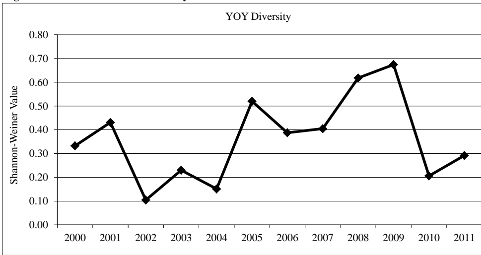
Figure A8-17. YOY whole lake diversity from 2000 to 2011.
