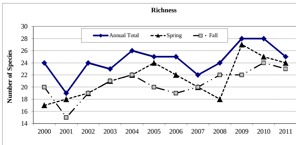
Figure A8-4. Electrofishing species richness in "all fish" transects from 2000-2011.
