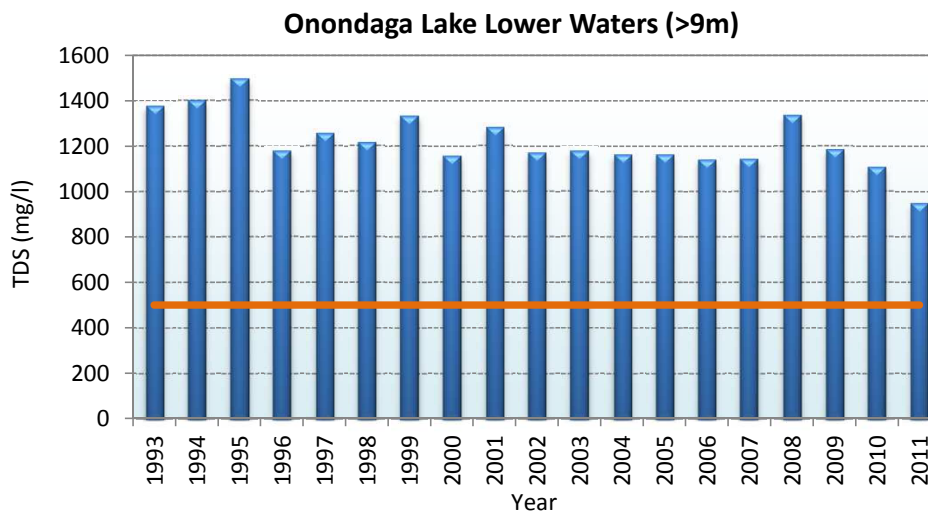
Time plot (1993- 2011) of Onondaga Lake South Deep station annual average total dissolved solids (TDS) concentrations in (a) upper (0-6m) depth average data, and (b) lower (>9m) depth average data . Annual average calculated using daily averages across multiple depths for some years. Ambient water quality standard (AWQS) of 500 mg/l.
