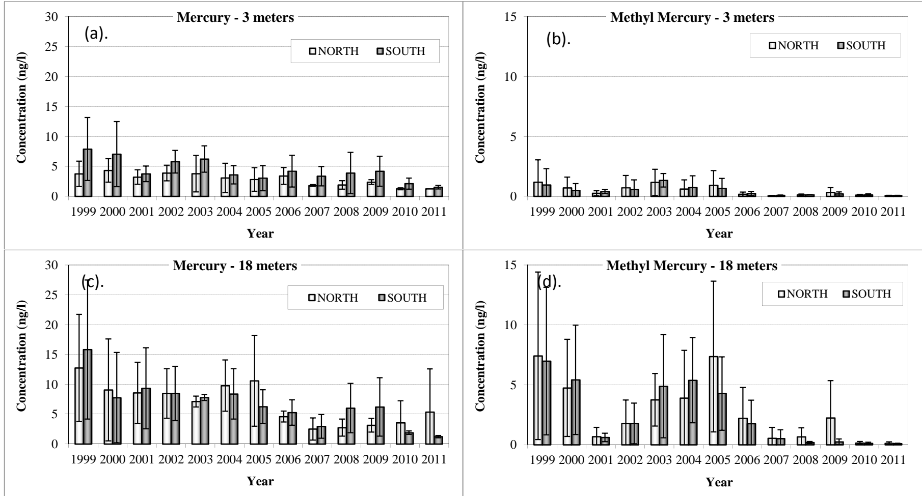
Time plot of the Onondaga Lake North and South Deep station annual average (a) 3 m mercury concentrations, (b) 3 m methyl-mercury concentrations, (c) 18 m mercury concentrations, (d) 18 m methyl-mercury concentration. The bars are the annual average based on 3 to six samples and the error bars are the standard deviations of the annual sampling.
