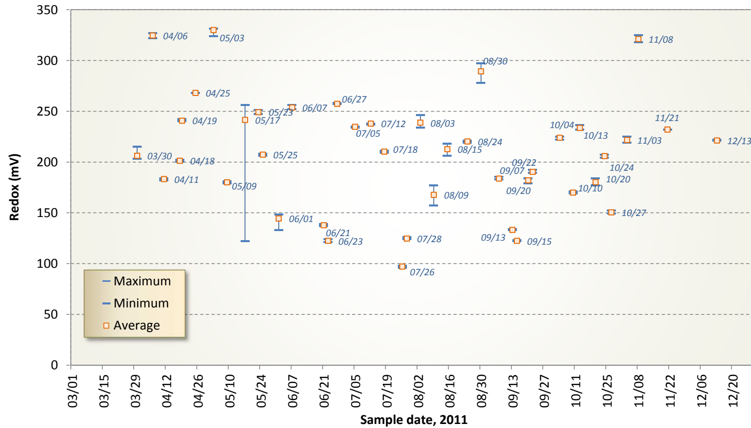
Statistical summary of redox, as measured during 2011 at Onondaga Lake South Deep station, depths \geq 15\text{m} . Measurements were taken every half-meter of depth (from 0-18.5m). The average, minimum and maximum redox for each sample date were calculated for the 15m through 18.5m measurements .
