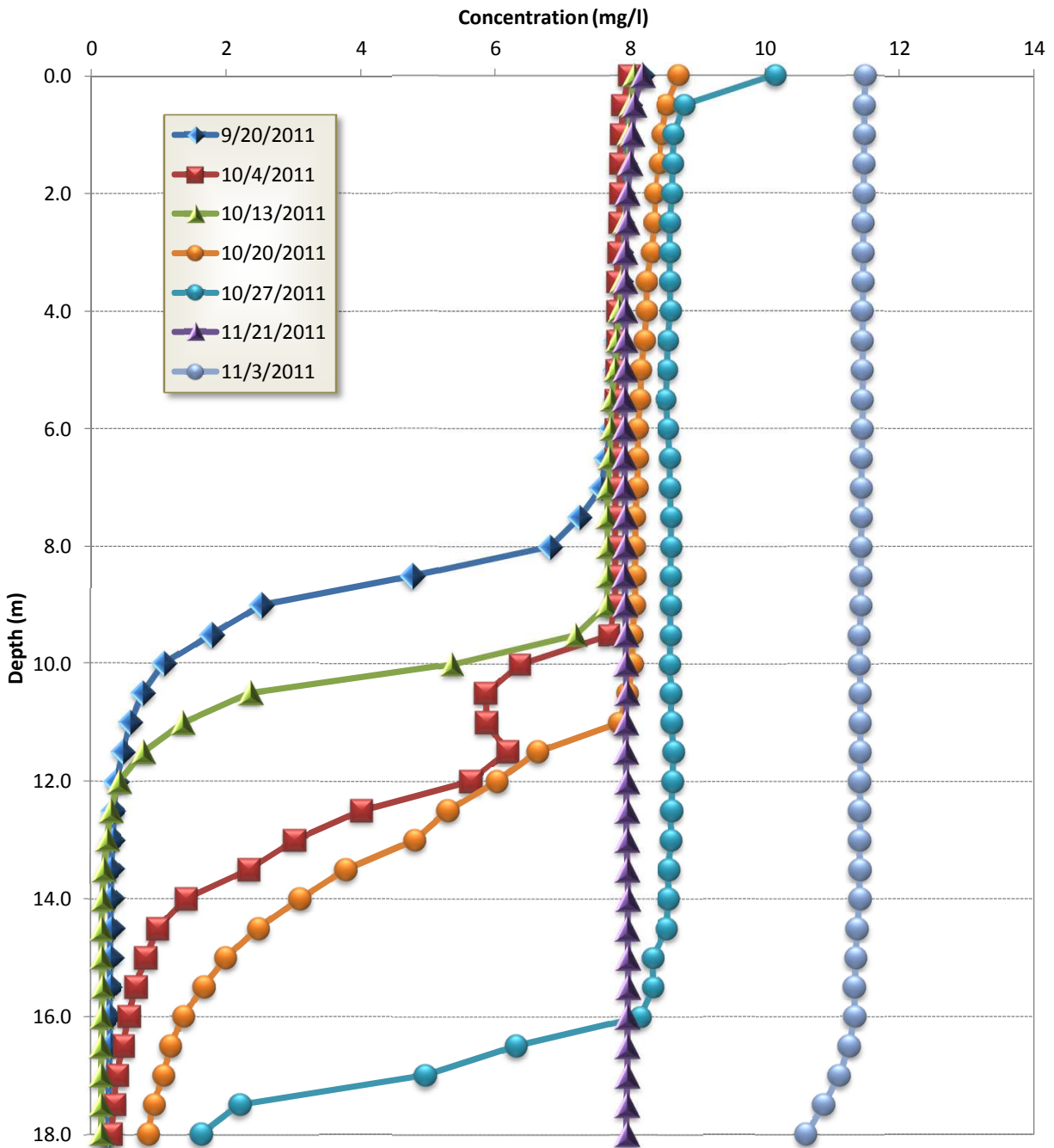
Field Dissolved Oxygen profiles collected biweekly at Onondaga Lake South Deep Station. This plots shows the progressive deepening of the thermocline In the fall of 2011. As the mixed layer moves down oxygen concentrations in the lower waters increases. Turnover occurred 11/3/2011 this year based on the biweekly temperature data (i.e., top to bottom temperatures difference was less then 1°C).
