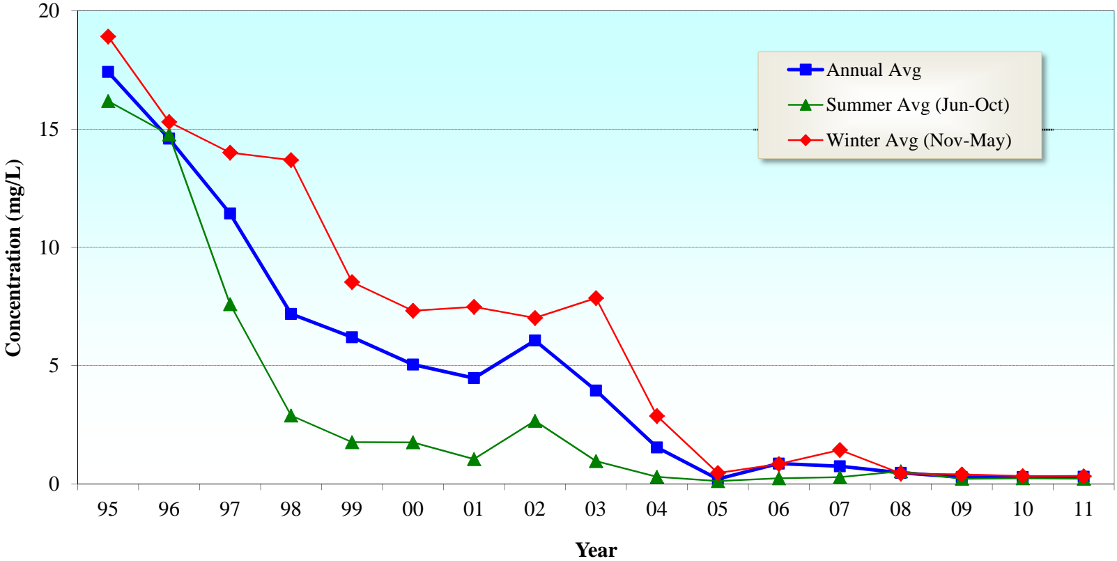
Time series of annual average and seasonal average (winter and summer) ammonia-N concentration in Metro Outfall 001 effluent over the 1995 through 2011 interval.
