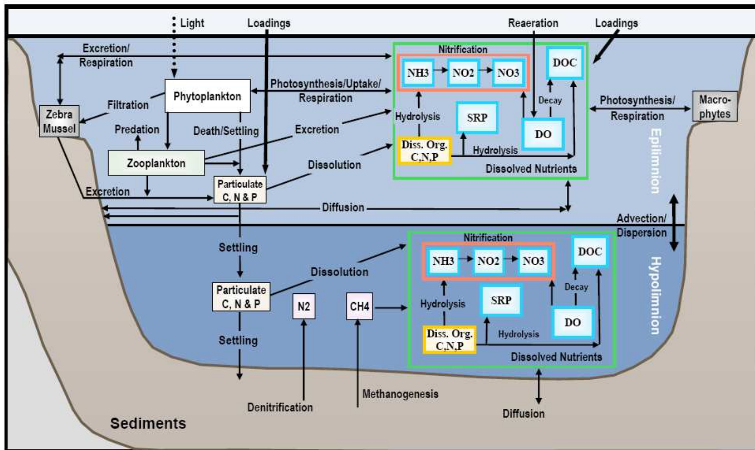
Conceptual diagram of major state variables and processes represented within the Onondaga Lake Water Quality Model (OLWQM).
